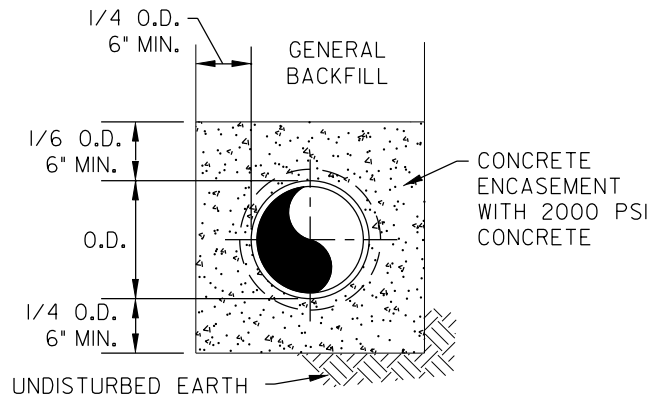
CONCRETE ENCASEMENT
