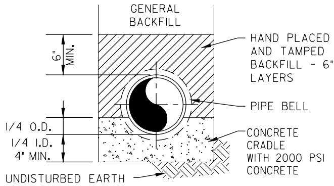
CLASS A CONCRETE CRADLE
