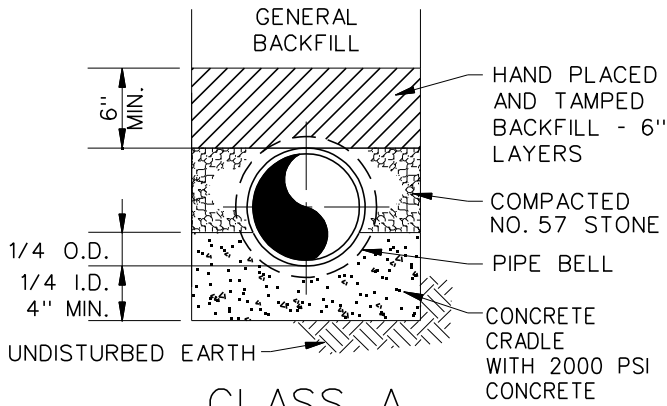
CLASS A CONCRETE CRADLE
