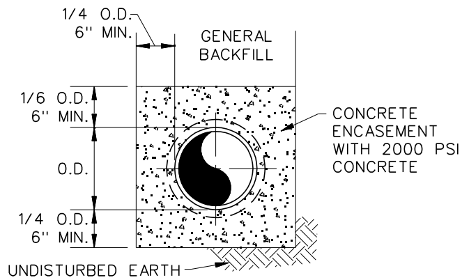
CONCRETE ENCASEMENT
