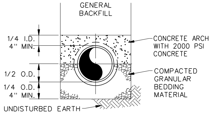
CLASS A CONCRETE ARCH
