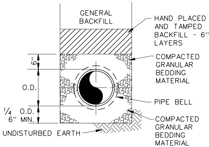
CLASS B - FOR PVC PIPE
